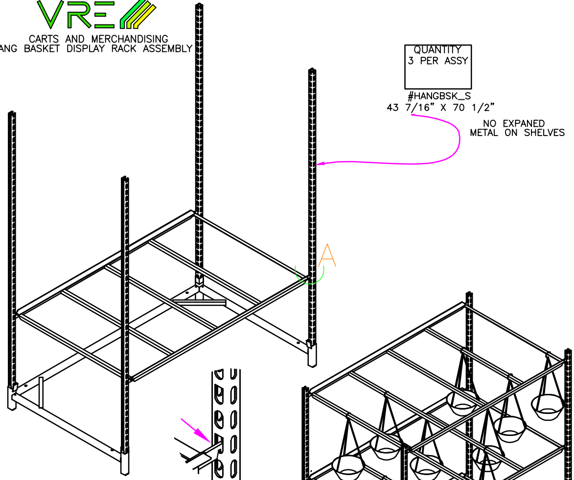
DETAIL A SHELF HOOK IN POLE
